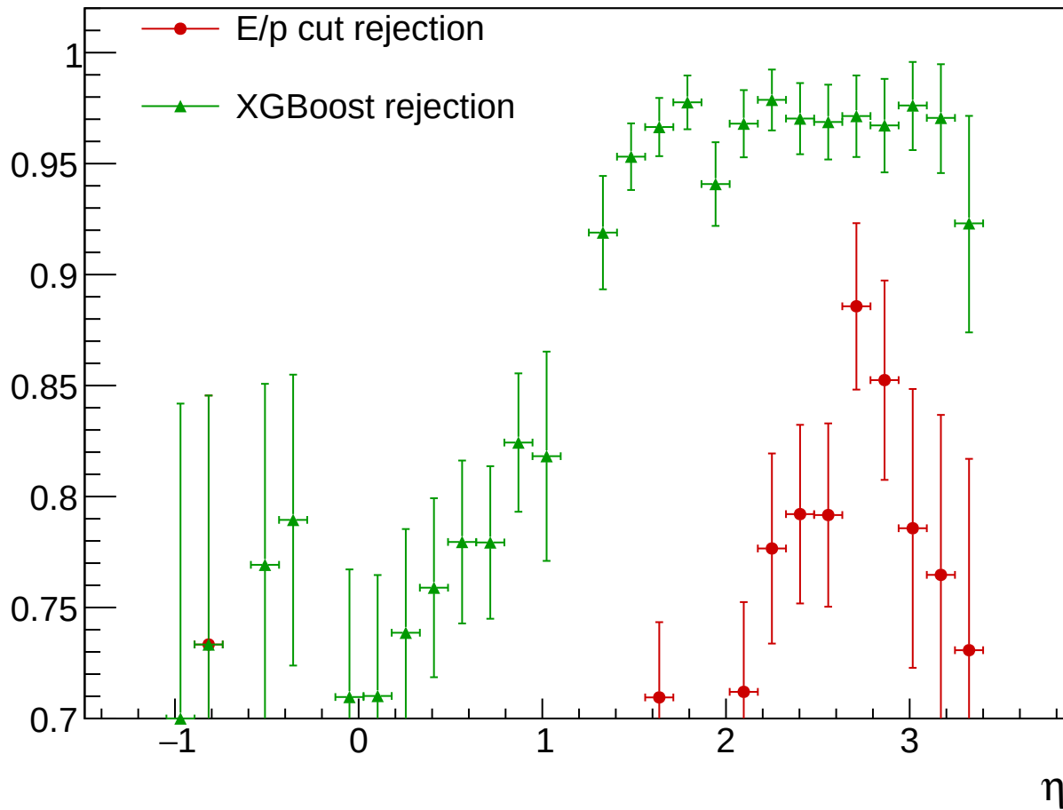
Pion Rejection vs \eta
