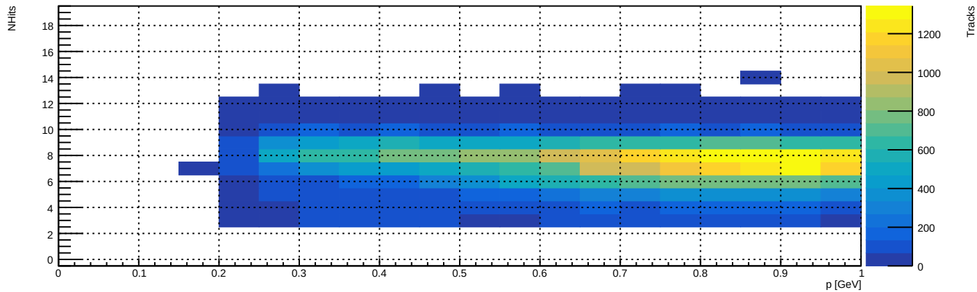
NHits vs P - Pion
