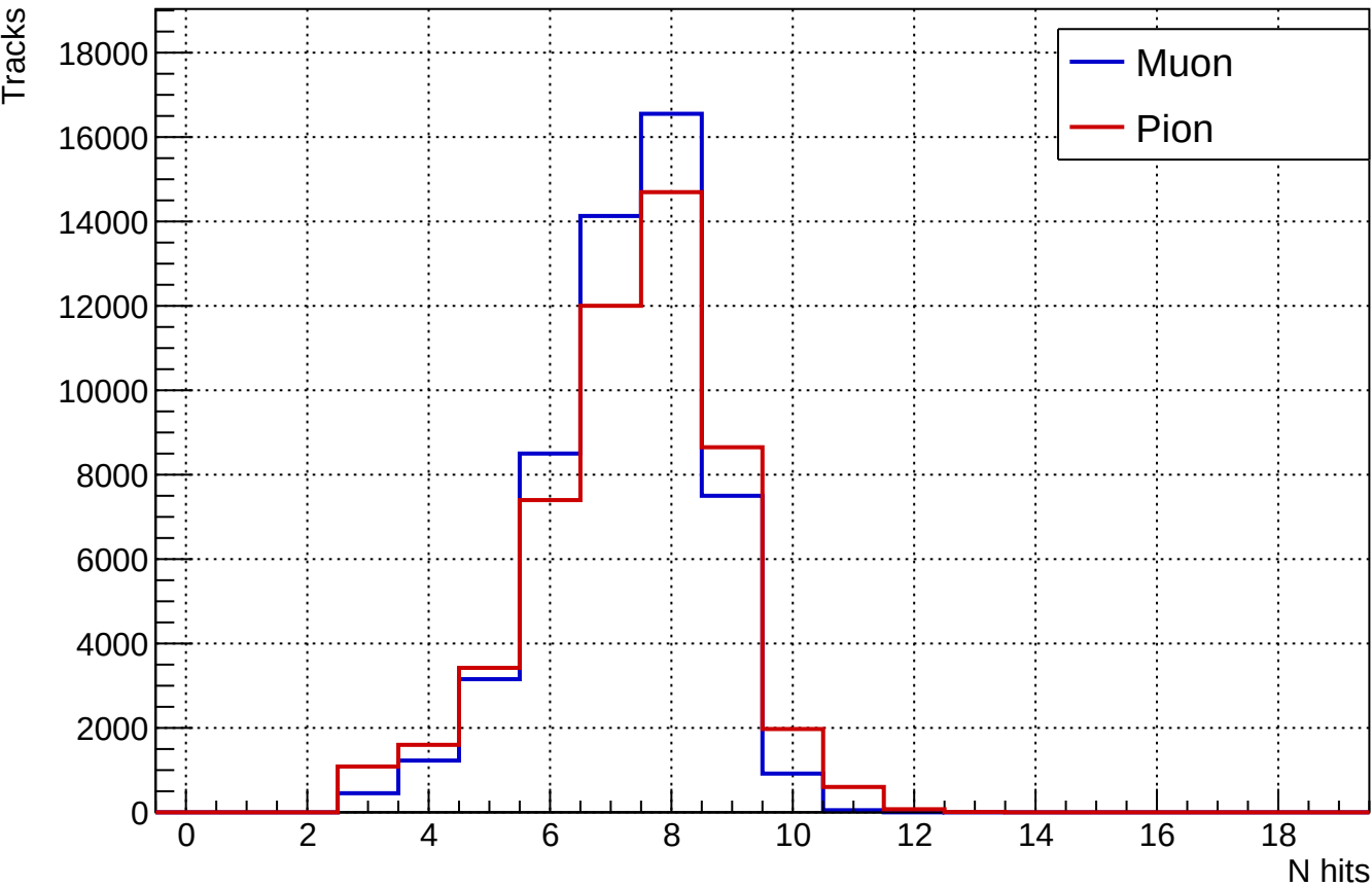
Number of hits in track
