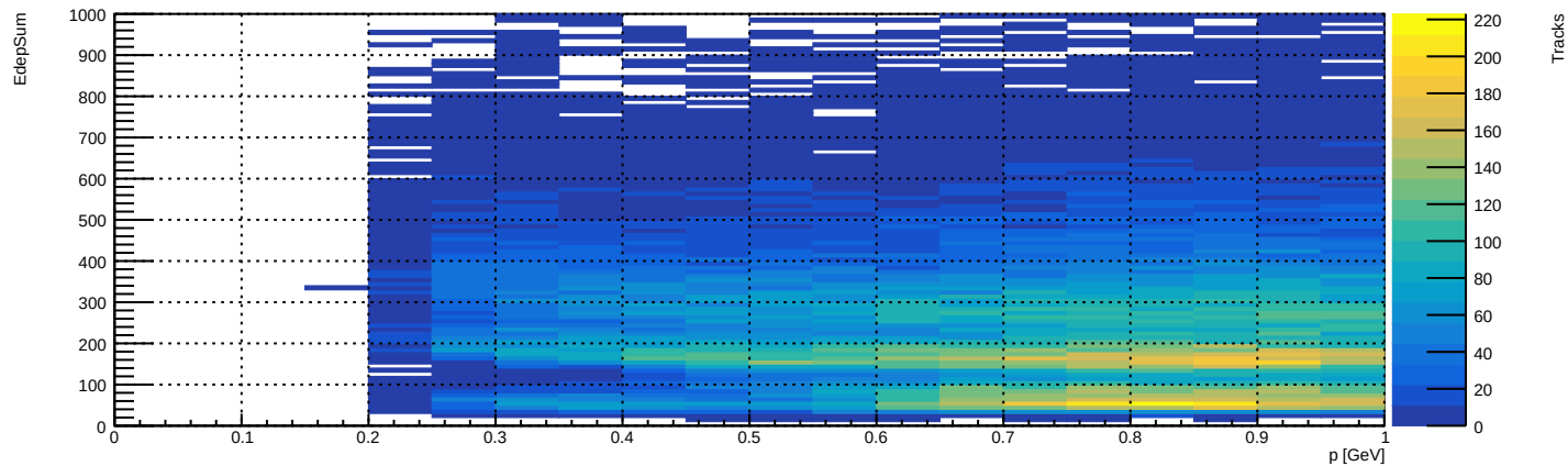
EdepSum vs P - Pion
