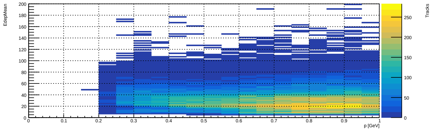
EdepMean vs P - Pion
