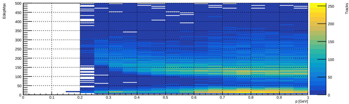
EdepMax vs P - Pion
