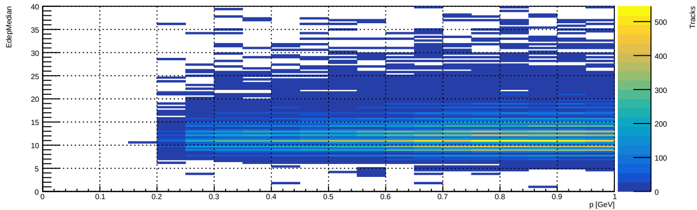
EdepMedian vs P - Pion
