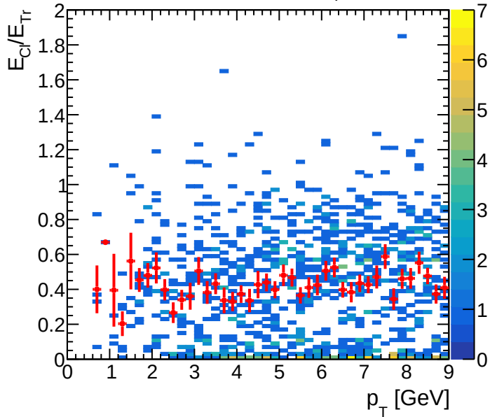
E_{\text{Cl}}/E_{\text{Tr}} vs track p_{\text{T}}
