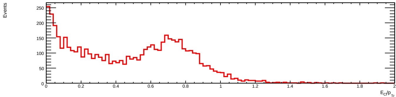
Cluster energy / track momentum
