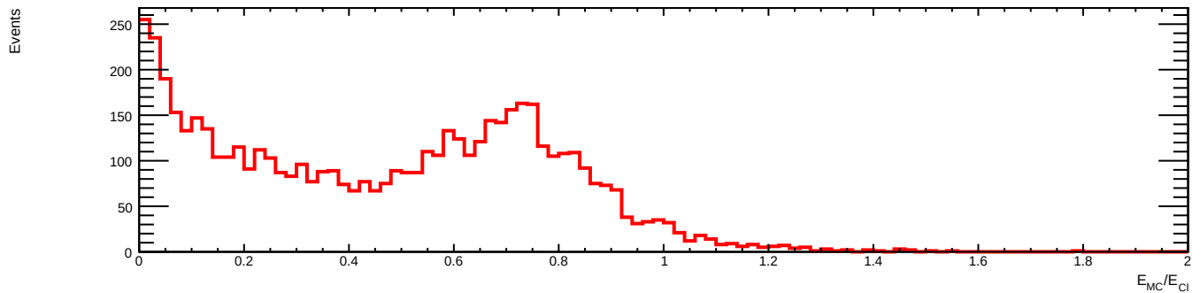
MC energy / cluster energy
