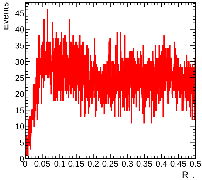
Matching distance R_{\eta\phi}
