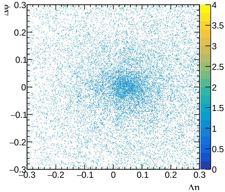
Cluster-Track matching \Delta\eta vs \Delta\phi
