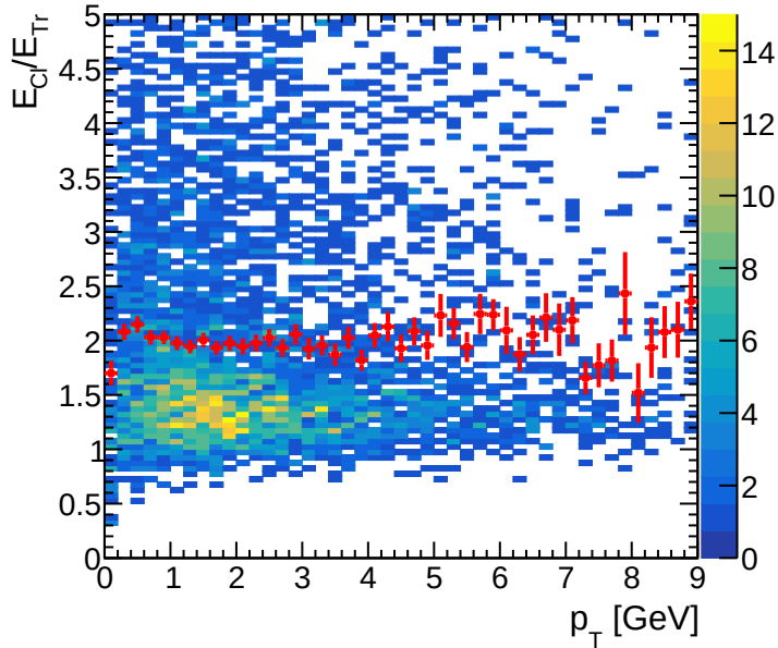
E_{\text{Cl}}/E_{\text{Tr}} vs track p_{\text{T}}
