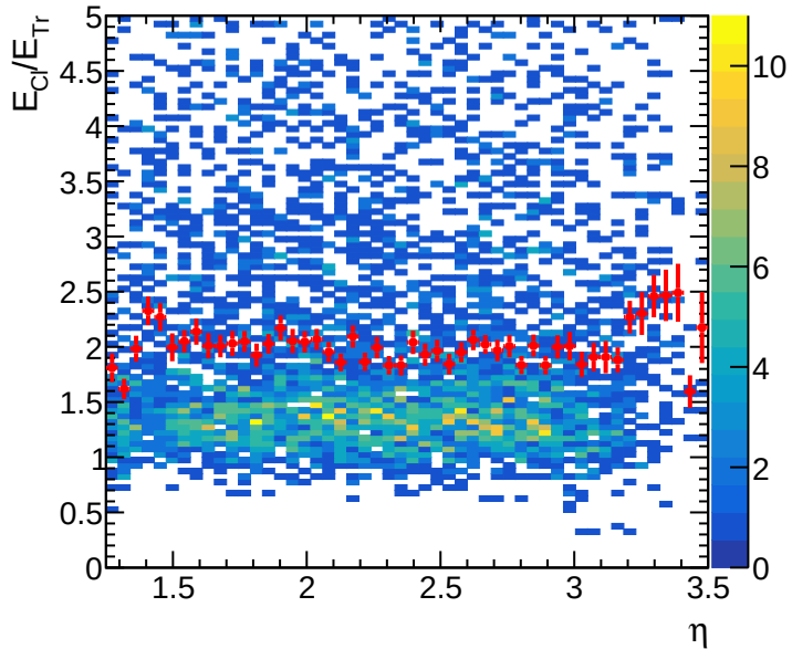
E_{\text{Cl}}/E_{\text{Tr}} vs track \eta
