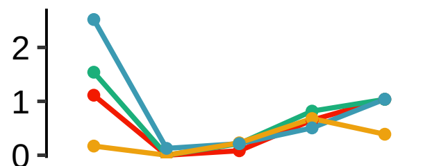
Unclassified DNA
