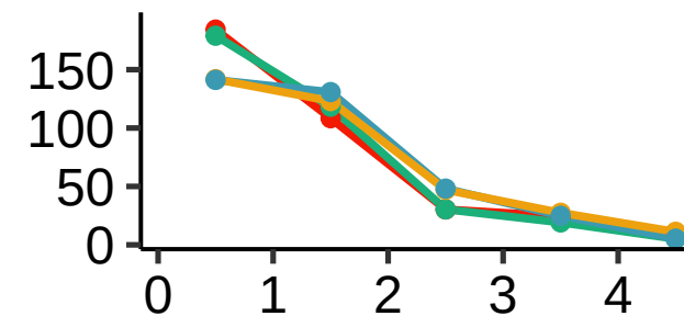
Jockey (LINE)
