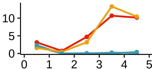
CR1-L2 (LINE)
