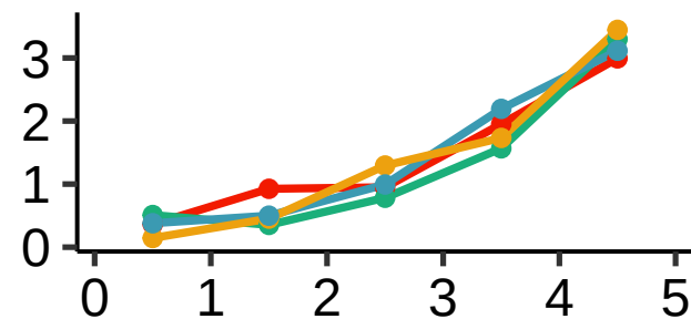
I-Jockey (LINE)
