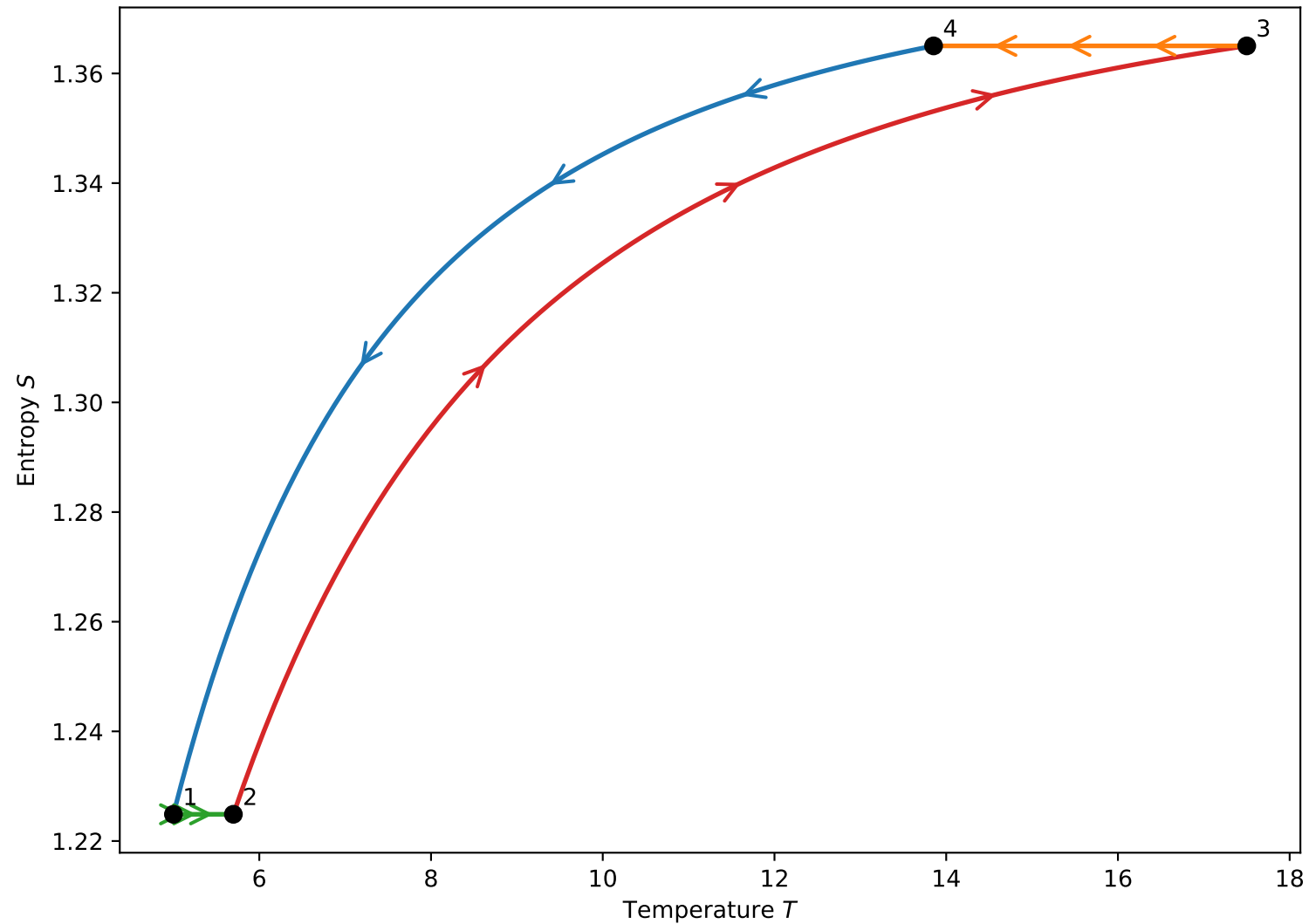
S \times T — Engine ( \eta = 0.169 )
