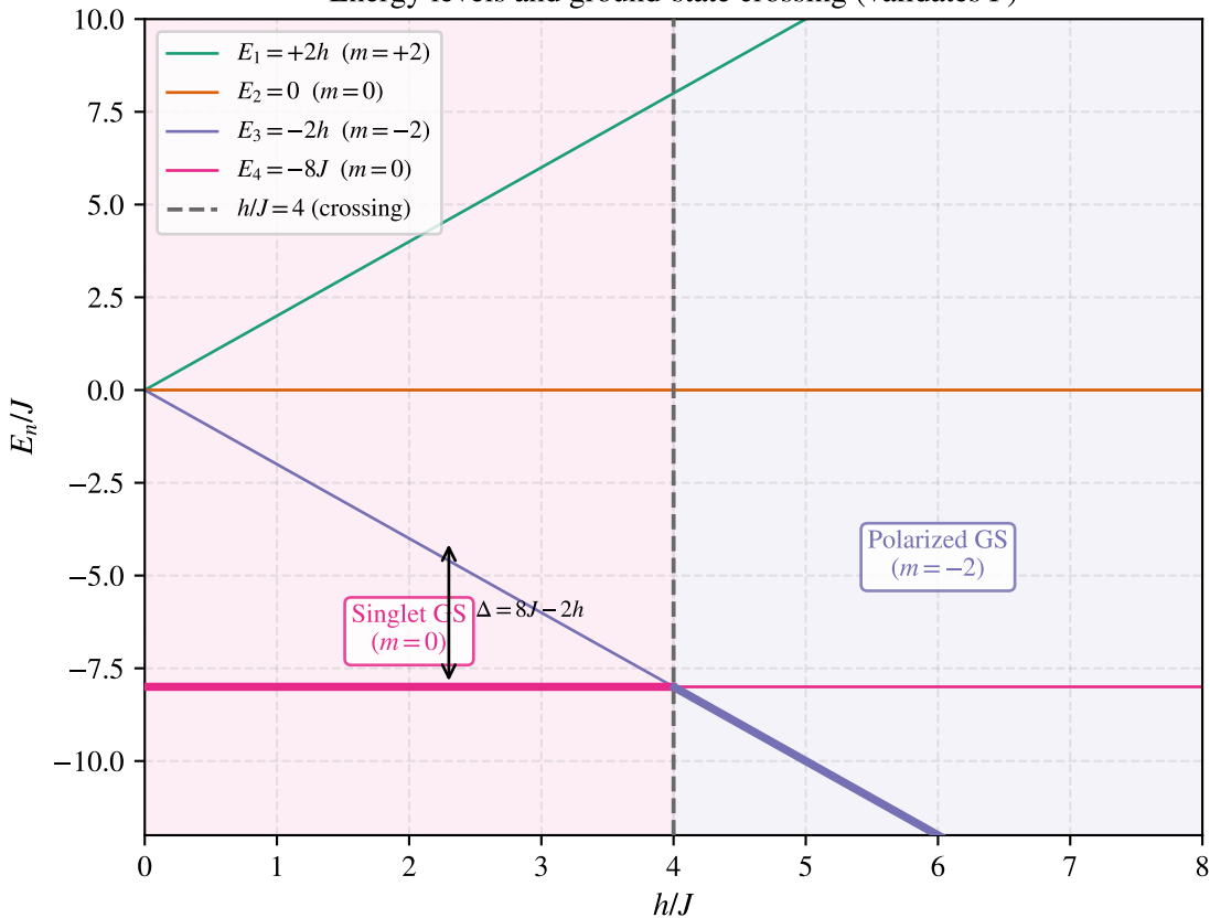
Energy levels and ground-state crossing (validates F)
