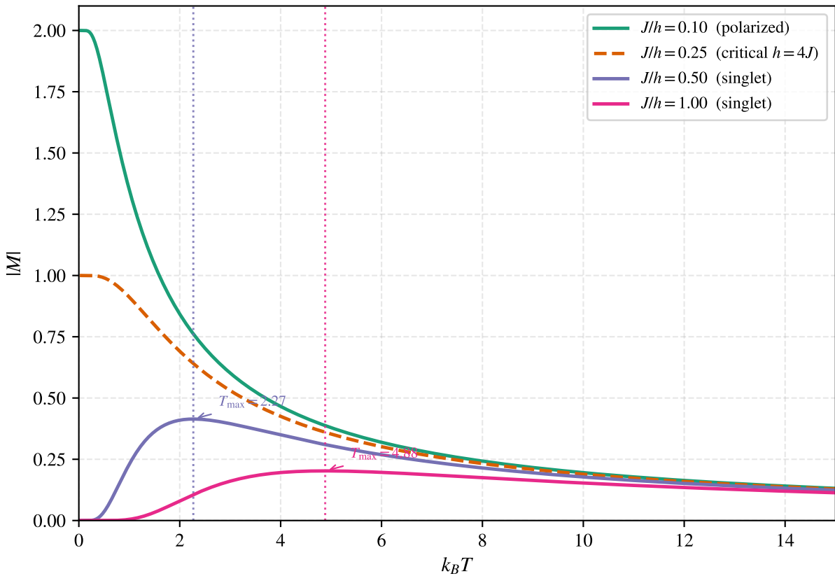
|M| vs T , fixed h=1 (validates B, C, D, E)
