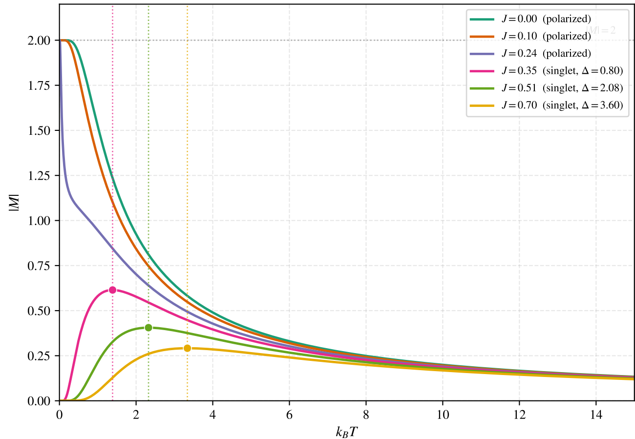
|M| vs T (fixed h = 1.0 , J_c = h/4 = 0.25 )
