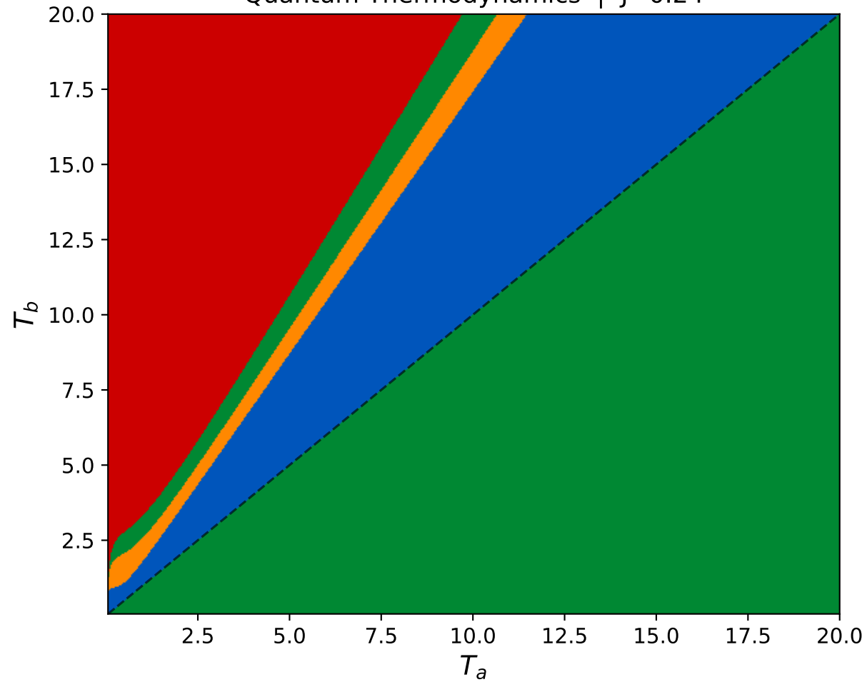
Quantum Thermodynamics | J=0.24
