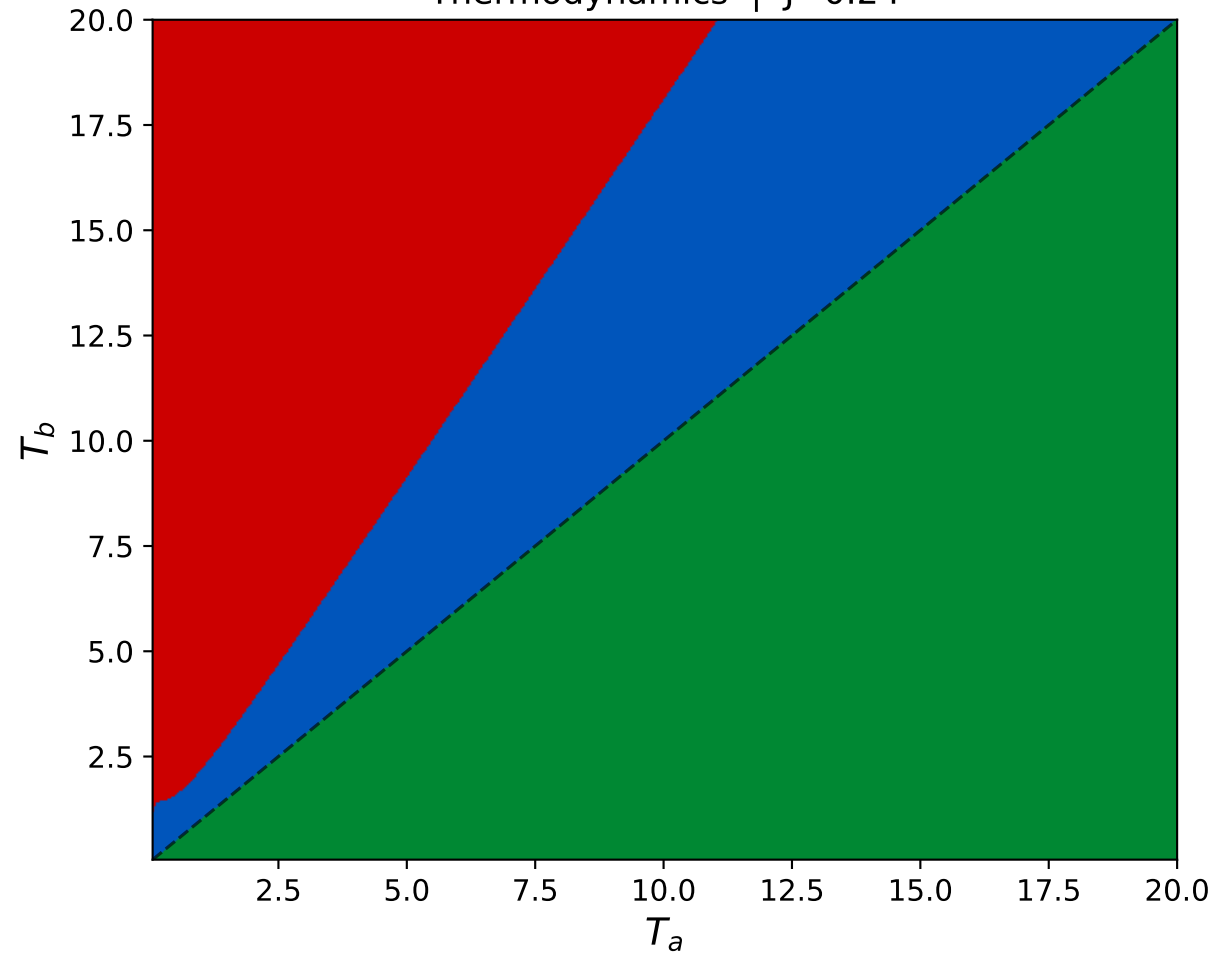
Thermodynamics | J=0.24
