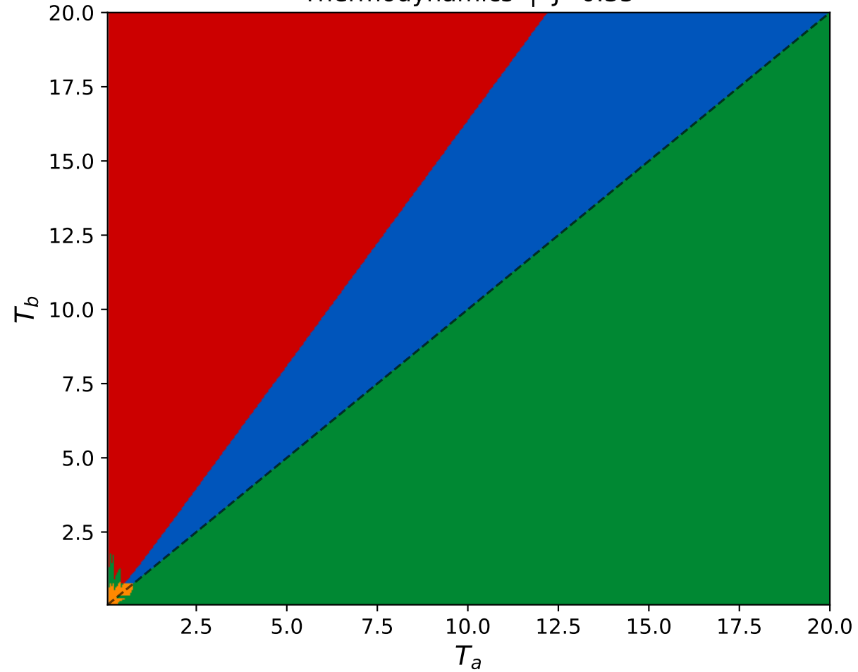
Thermodynamics | J=0.35
