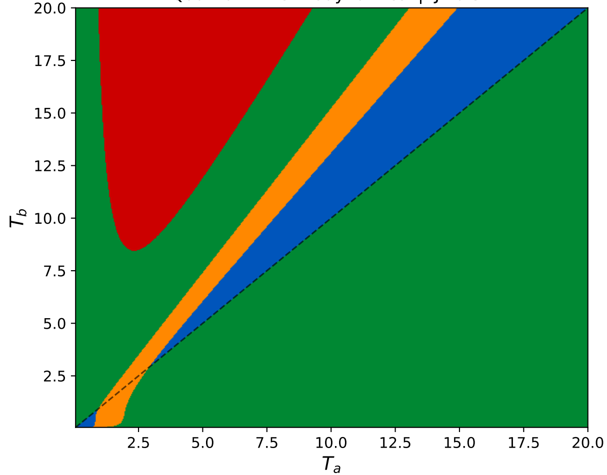
Quantum Thermodynamics | J=0.51
