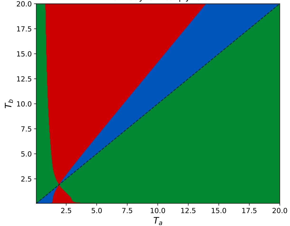
Thermodynamics | J=0.51
