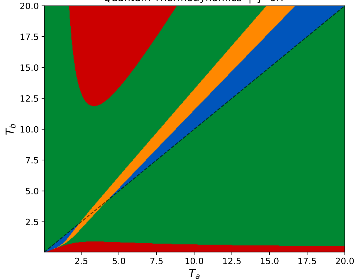
Quantum Thermodynamics | J=0.7
