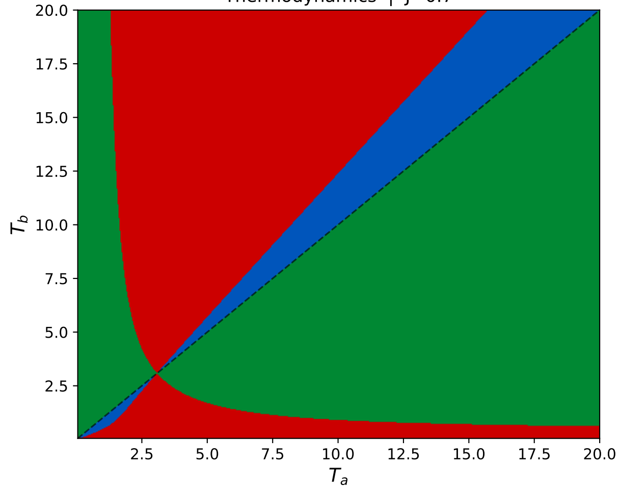
Thermodynamics | J=0.7
