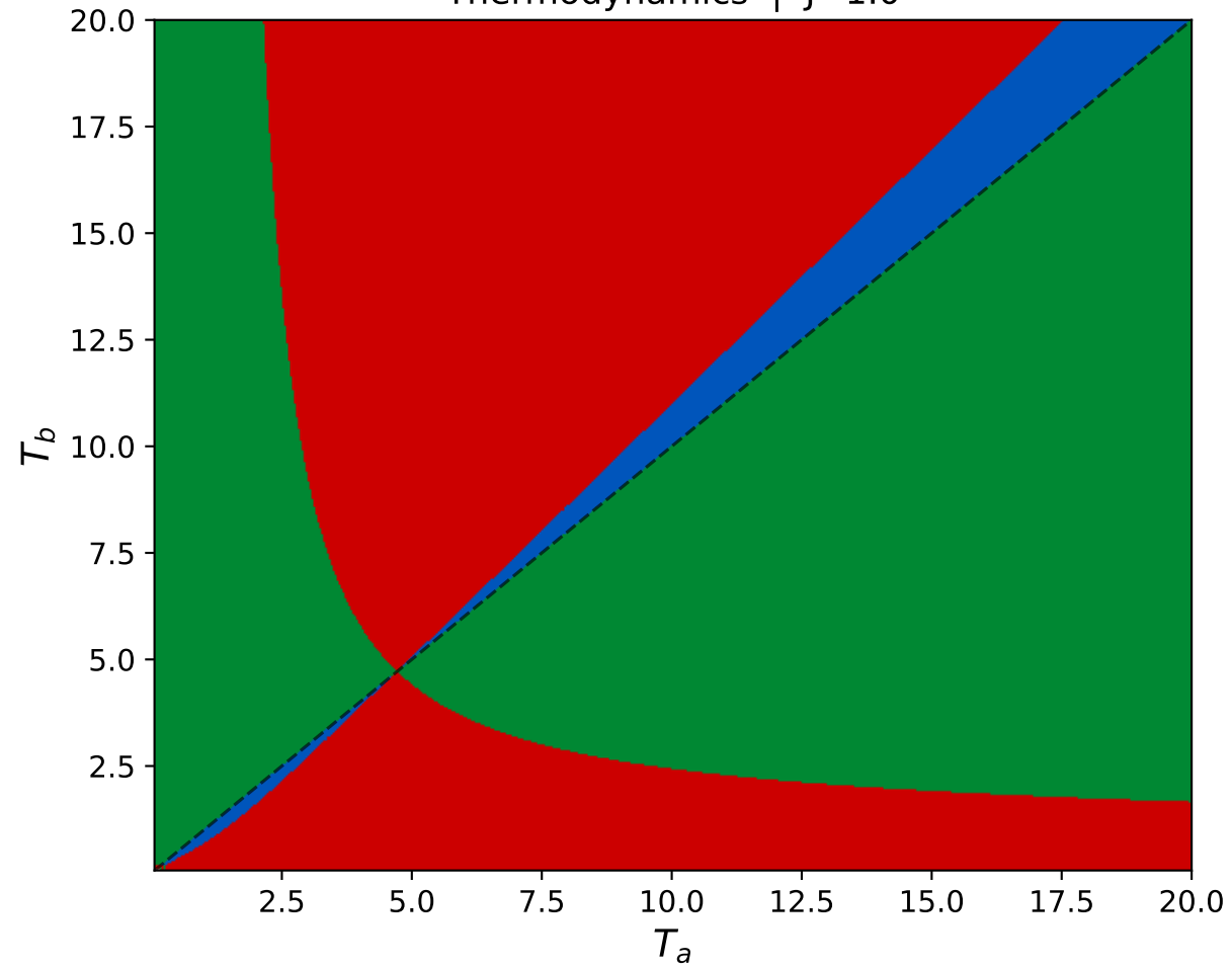
Thermodynamics | J=1.0
