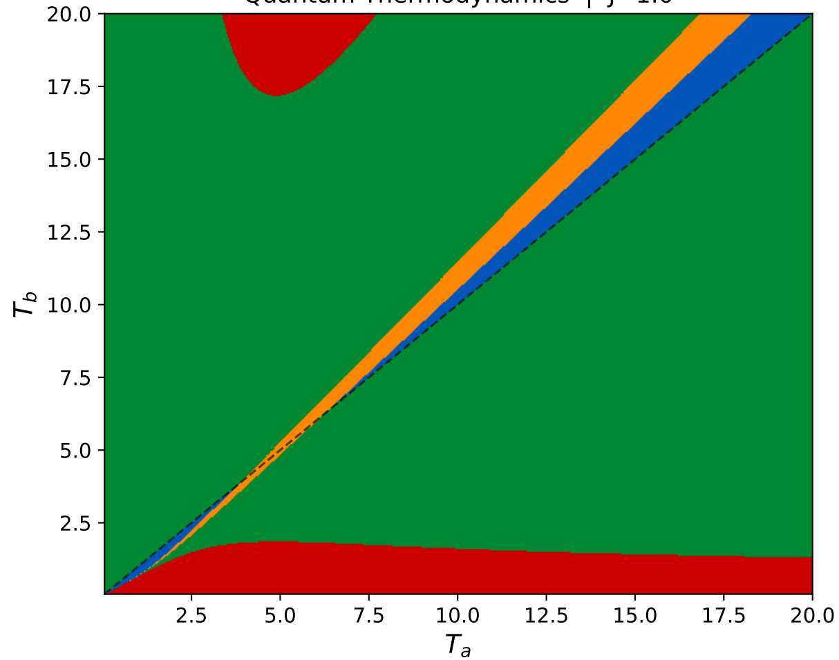
Quantum Thermodynamics | J=1.0
