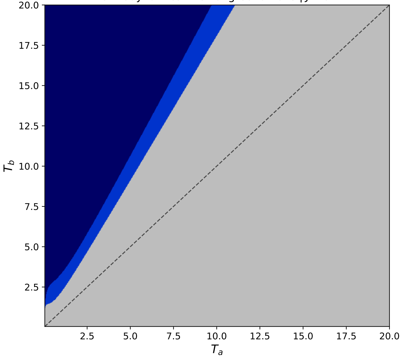
Thermodynamics — Strong Conditions |J| = 0.24
