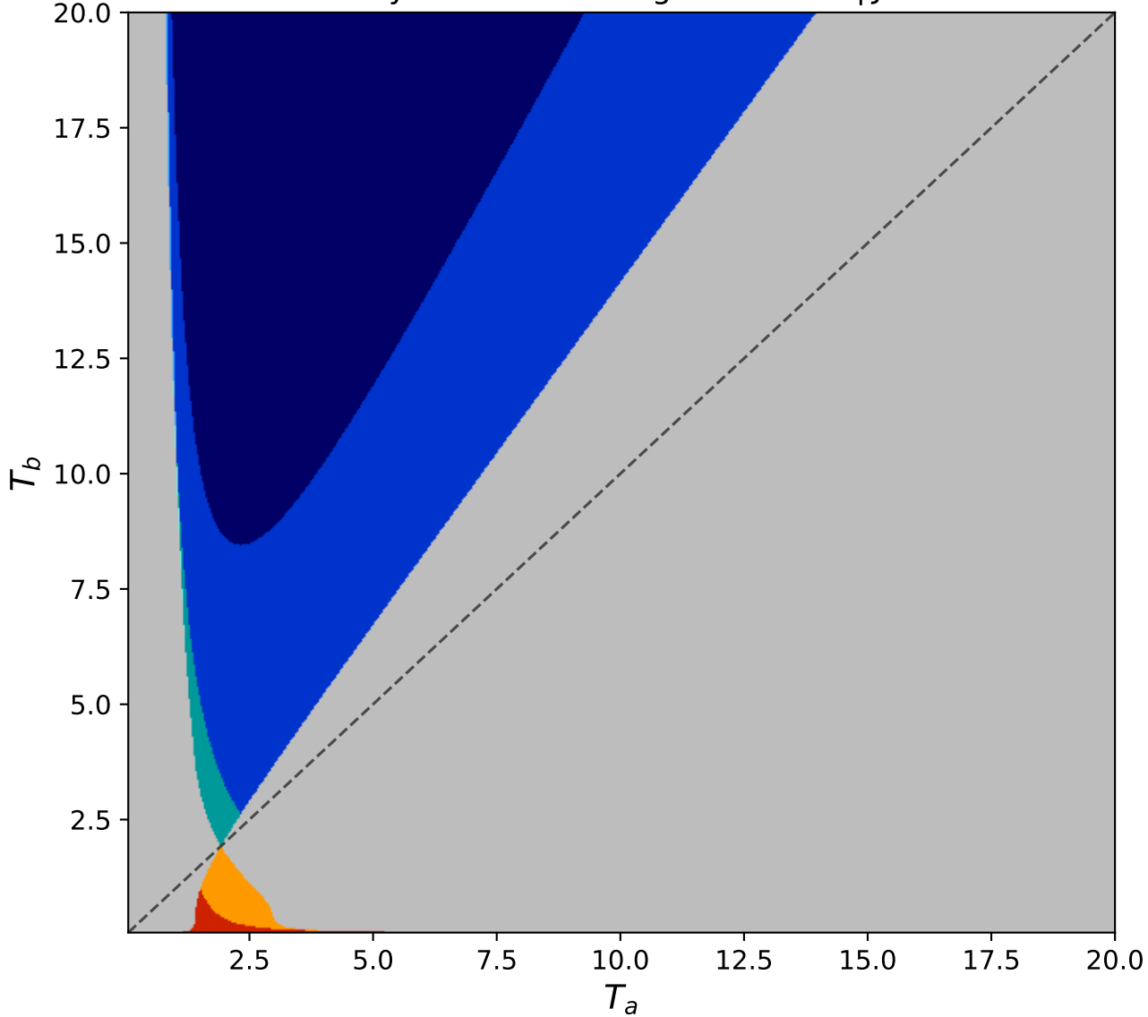
Thermodynamics — Strong Conditions |J| = 0.51
