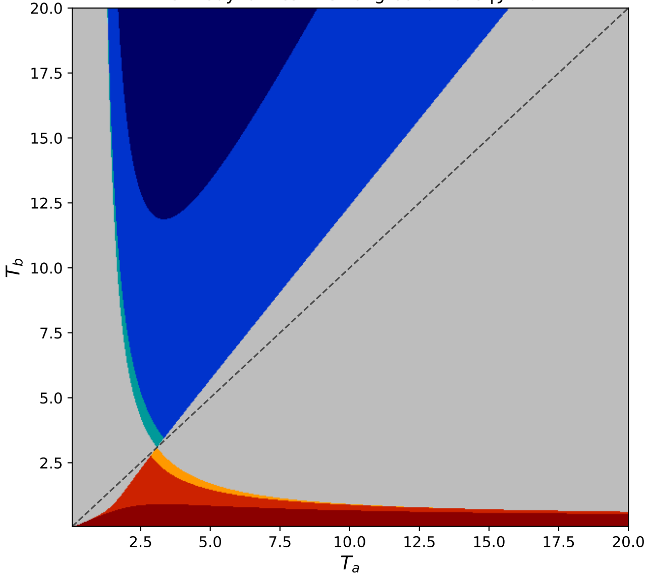
Thermodynamics — Strong Conditions |J| = 0.7
