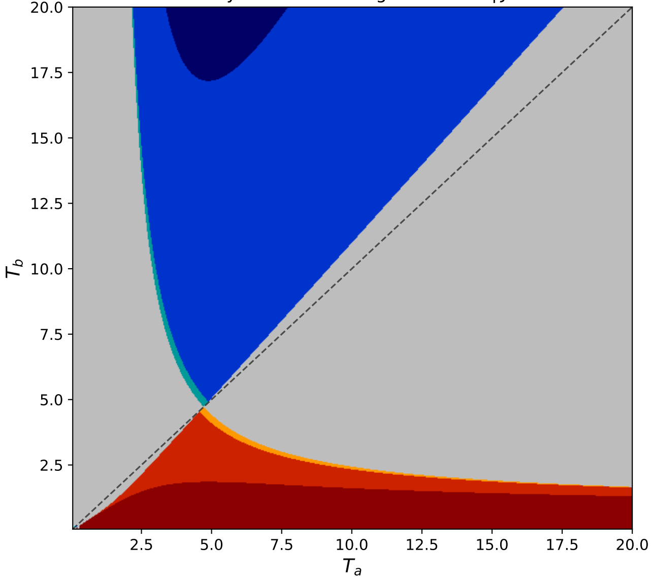
Thermodynamics — Strong Conditions |J| = 1.0
