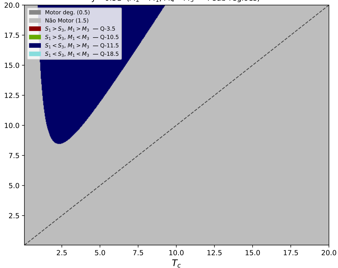
Quantum Thermodynamics — Strong J = 0.51 ( M_2 = M_1, M_4 = M_3 \rightarrow 4 sub-regiões)
