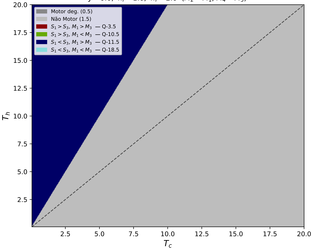
Quantum — Strong Conditions J = 0.0, \quad h_i = 1.0, \quad h_f = 2.0 \quad (M_2 = M_1, M_4 = M_3)
