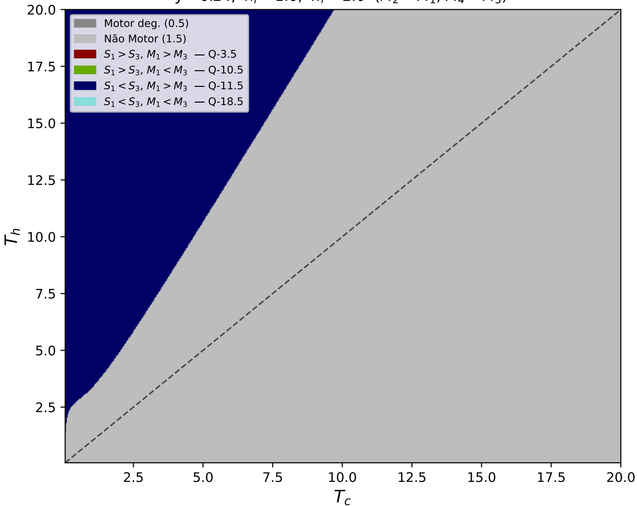
Quantum — Strong Conditions J = 0.24, h_i = 1.0, h_f = 2.0 ( M_2 = M_1, M_4 = M_3 )
