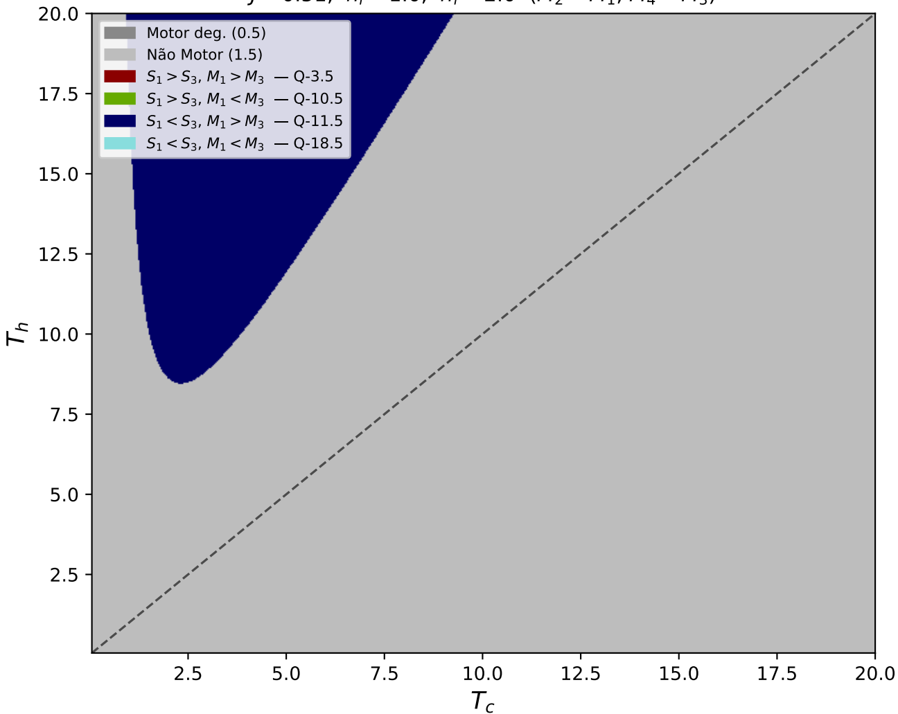
Quantum — Strong Conditions J = 0.51, h_i = 1.0, h_f = 2.0 ( M_2 = M_1, M_4 = M_3 )
