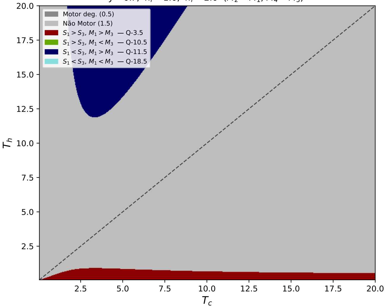
Quantum — Strong Conditions J = 0.7, \quad h_i = 1.0, \quad h_f = 2.0 \quad (M_2 = M_1, M_4 = M_3)
