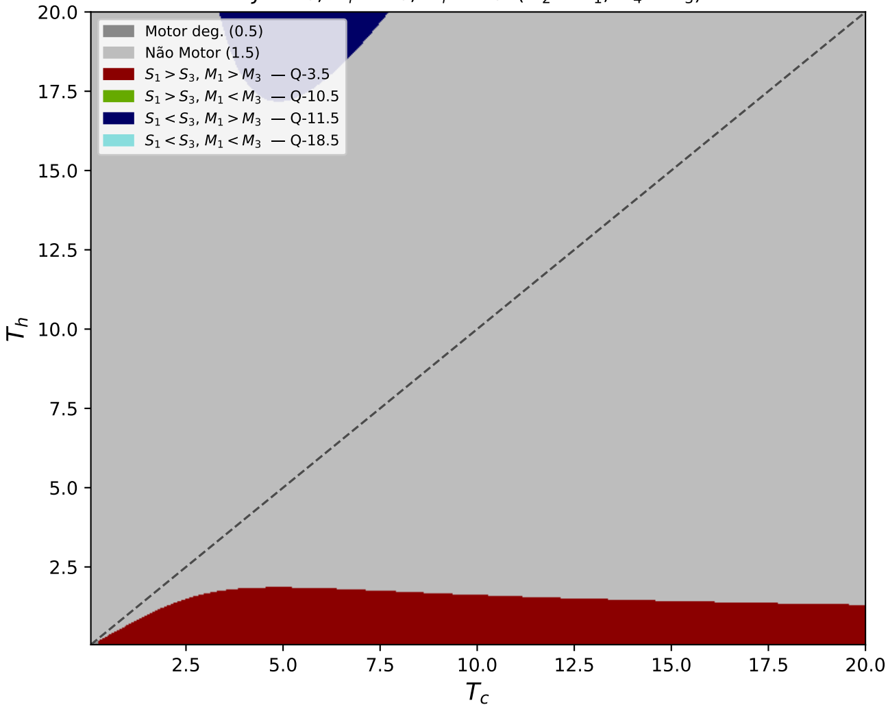
Quantum — Strong Conditions J = 1.0, h_i = 1.0, h_f = 2.0 ( M_2 = M_1, M_4 = M_3 )
