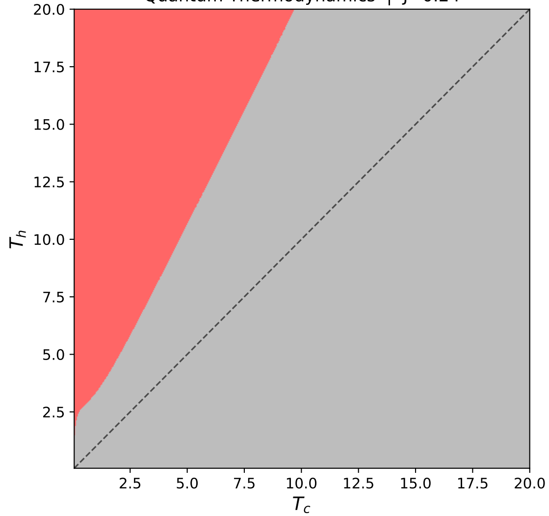
Quantum Thermodynamics | J=0.24
