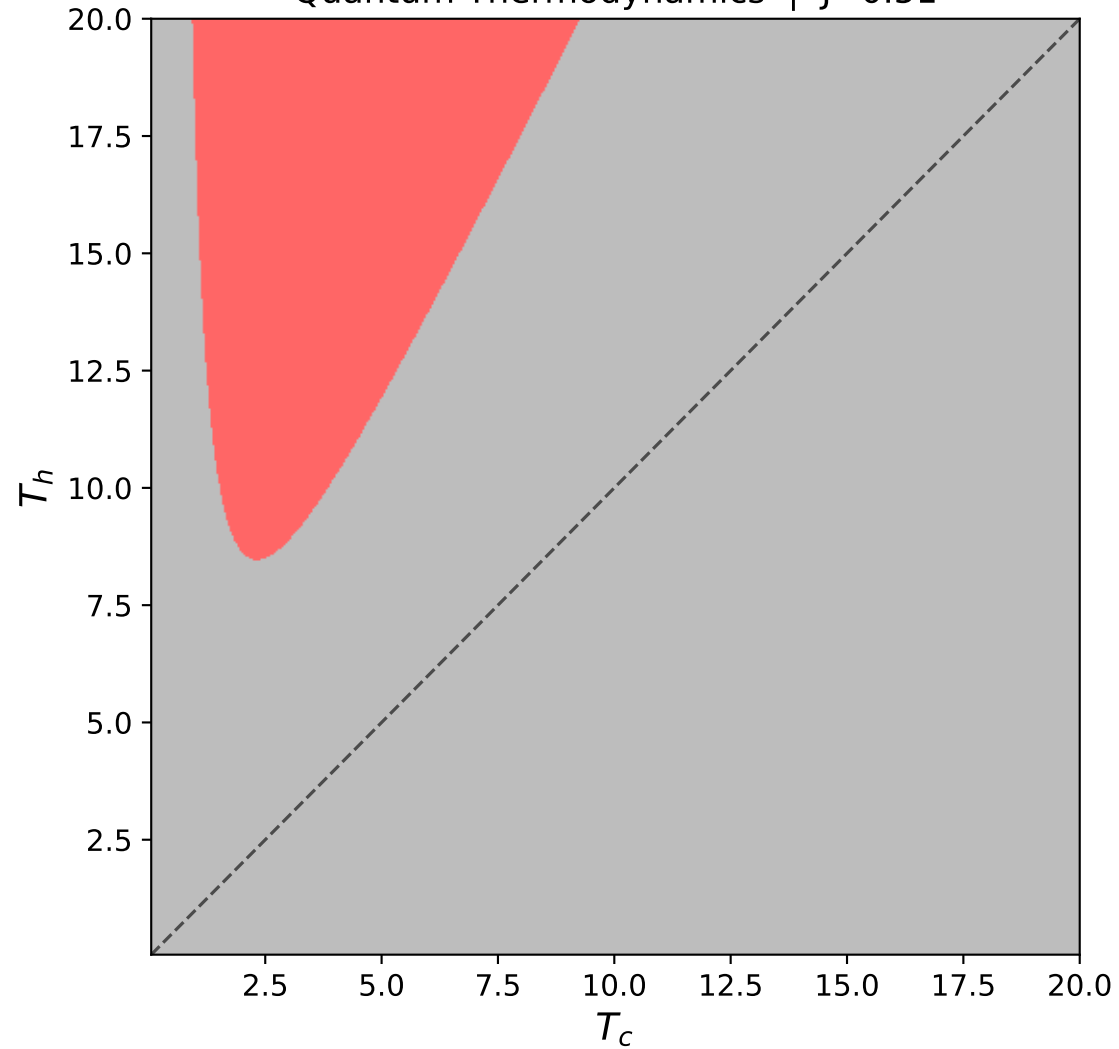
Quantum Thermodynamics | J=0.51
