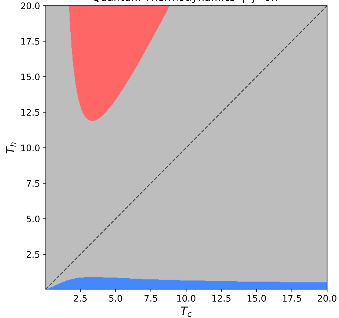
Quantum Thermodynamics | J=0.7
