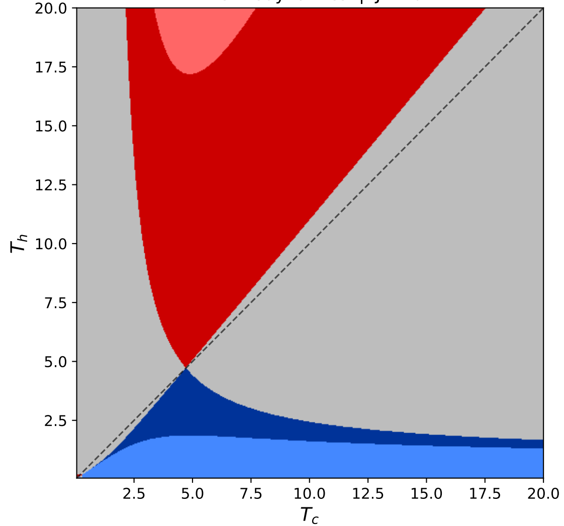
Thermodynamics | J=1.0
