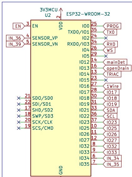
ESP32-Wroom32
