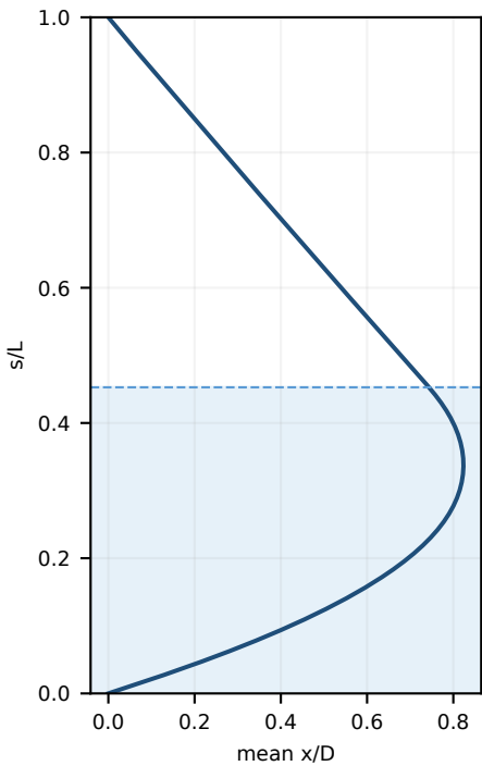
Chaplin-style simulated response; late representative CF period
