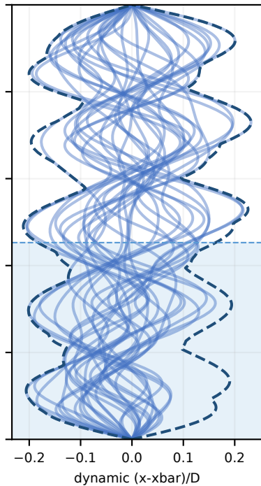
Chaplin-style simulated response; late representative CF period
