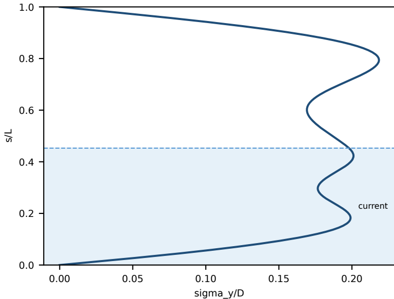
Cross-flow RMS (0-10s)
