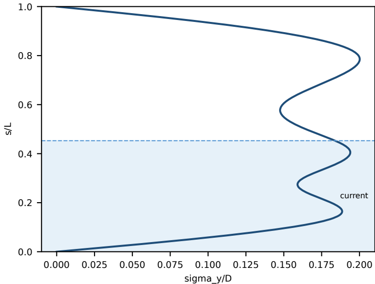
Cross-flow RMS (5-10s)
