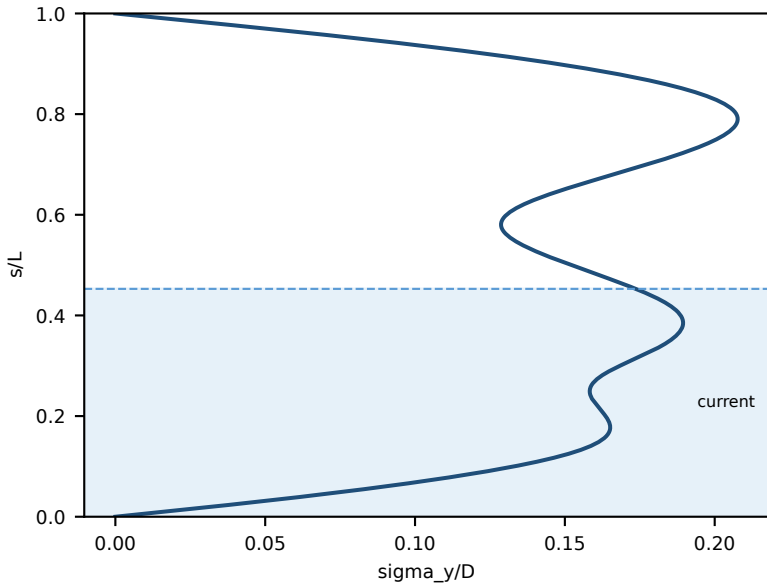
Cross-flow RMS (7.5-10s)
