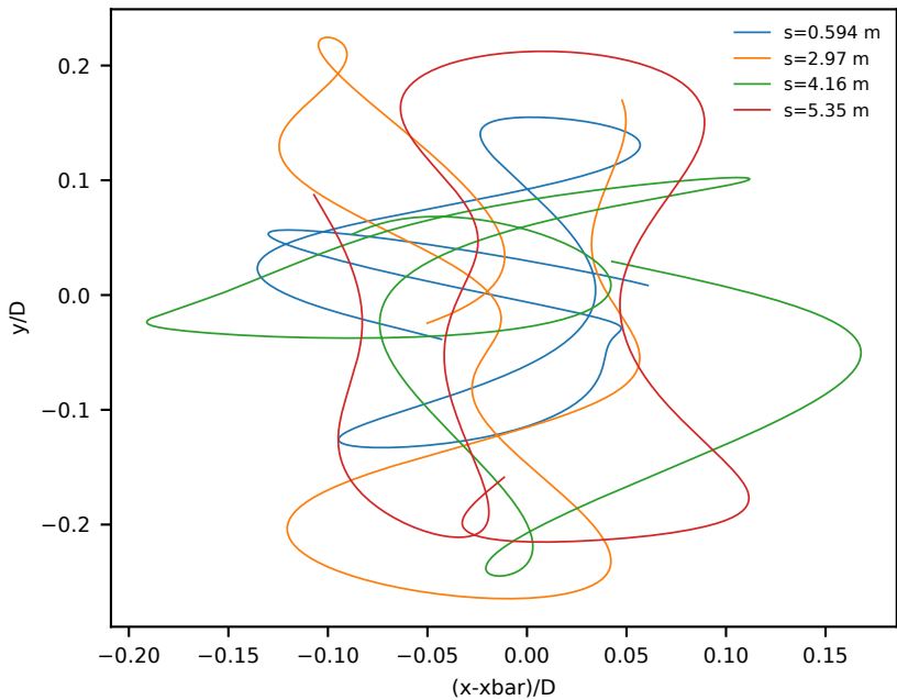
Late XY trajectories: 5-10s, 1 CF period(s)
