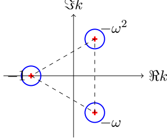
Figure 1: The cyclic cubic family has three exceptional points forming an equilateral triangle. Under w = k^3 + 1 , each small meridian maps to a positive meridian around 0 in the w -plane.
