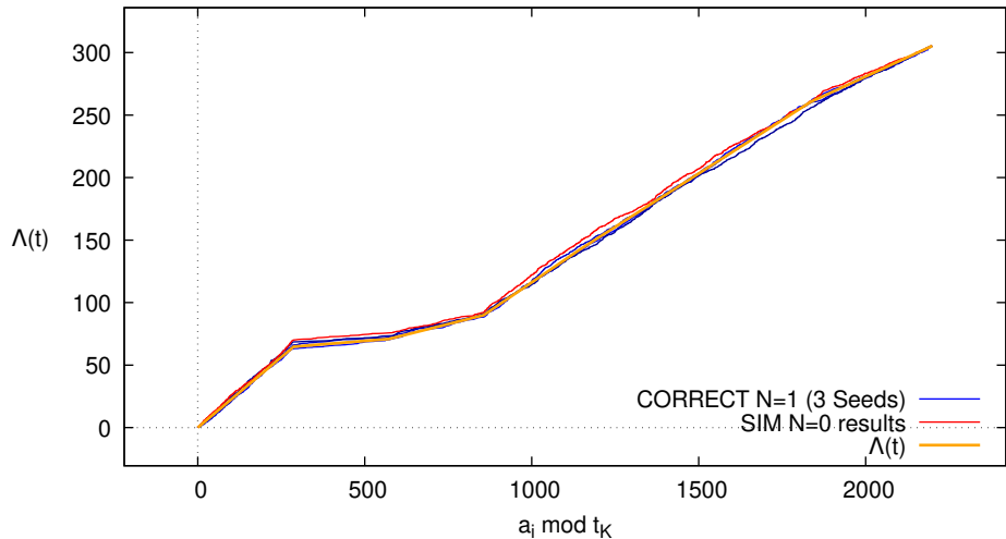
Piecewise Constant Non-stationary Arrivals (A.dat Q=30500)
