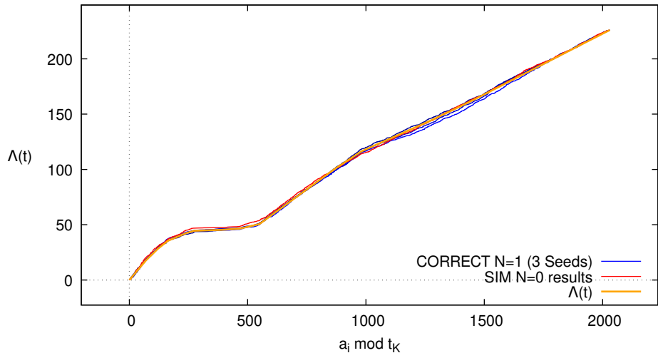
Piecewise Constant Non-stationary Arrivals (B.dat Q=22600)
