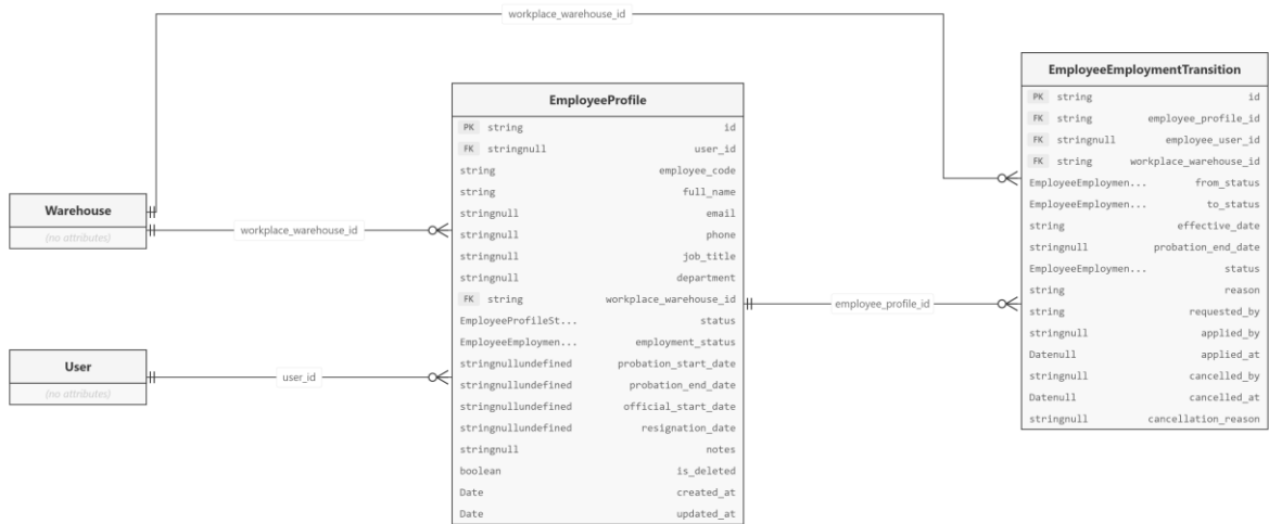
Hình 5-3:Entity Relationship Diagram Employee Profiles operations
