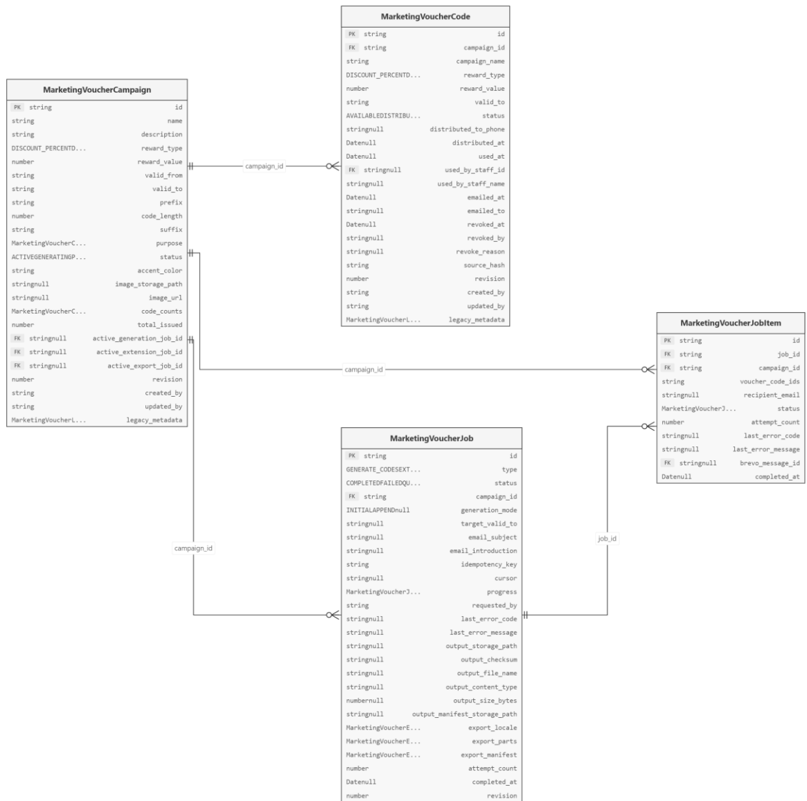
Hình 5-10: Entity Relationship Diagram Marketing Vouchers operations
