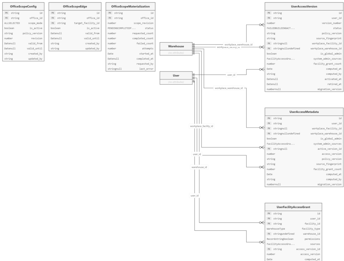
Hình 5-5: Entity Relationship Diagram Facility Access operations
