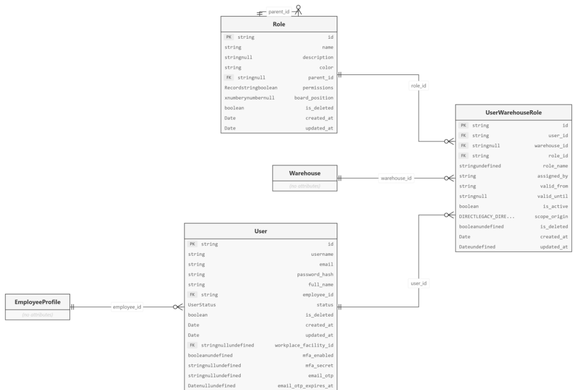
Hình 5-19: Entity Relationship Diagram Users operations
