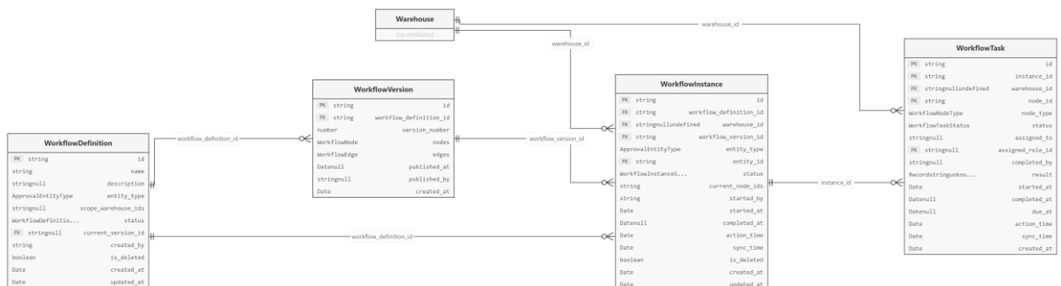
Hình 5-21: Entity Relationship Diagram Workflow operations
