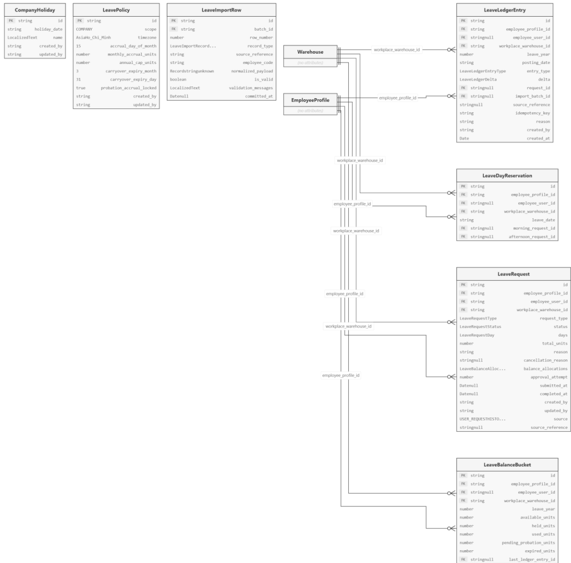
Hình 5-8: Entity Relationship Diagram Leave operations
