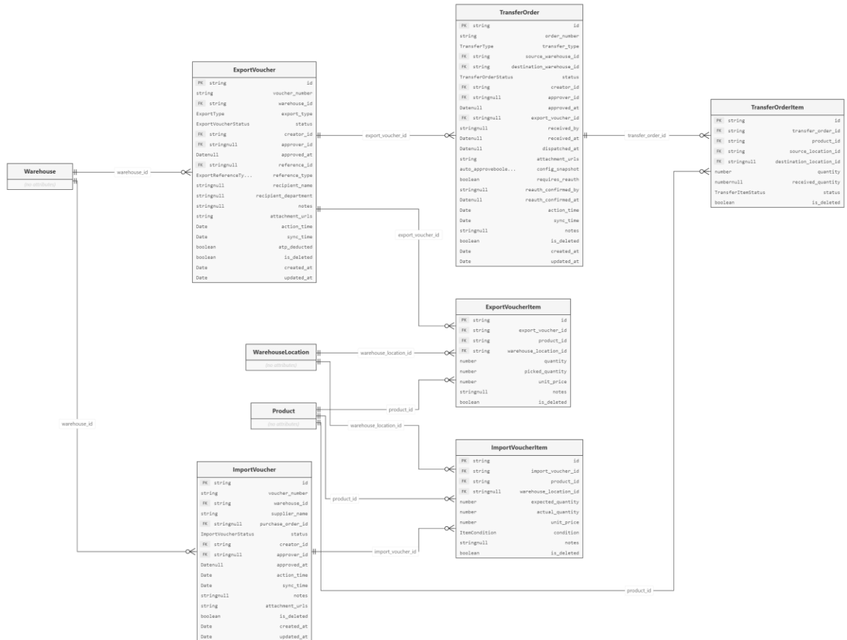
Hình 5-20: Entity Relationship Diagram Vouchers operations
