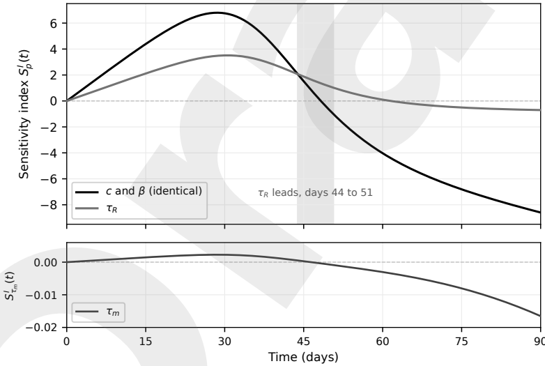
Figure 4.1. Computed time-dependent sensitivity indices S_p^I(t) for the SIR model at the nominal parameters of this chapter ( c = 5 , \beta = 0.06 , \tau_R = 7 , \tau_m = 10^4 , N = 1000 ). The indices for c and \beta are equal to machine precision, differing by about 10^{-15} , and are drawn as a single curve: the two POIs enter only through the product c\beta , so no computation can separate them. Both peak at 6.799 near day 29 and cross zero at day 48. The mean infectious period \tau_R peaks later, at 3.513 near day 31, and crosses zero at day 62. It leads only in the shaded window, days 44 to 51, around the epidemic peak; before and after it, transmission dominates. The mean residence time \tau_m is three orders of magnitude smaller and so is given its own panel with its own zero line; it changes sign at day 46 rather than staying negative throughout. Generated by generate_fig_sir_timevarySI.py , which reproduces these values byte for byte.
