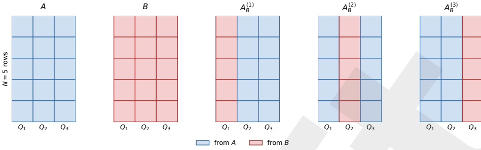
Figure 9.2. Saltelli pick-freeze matrix structure for m = 3 parameters (columns) and N = 5 sample rows. Blue cells carry values from the base matrix A ; red cells carry values from the independent matrix B . A_B^{(i)} shares every column with A except column i , which is “frozen” from B . This design ensures that A_B^{(i)} and A differ only in parameter Q_i , isolating Q_i ’s variance contribution from all interaction effects. The total cost is N(m + 2) model evaluations: N for A , N for B , and N for each of the m hybrid matrices.
