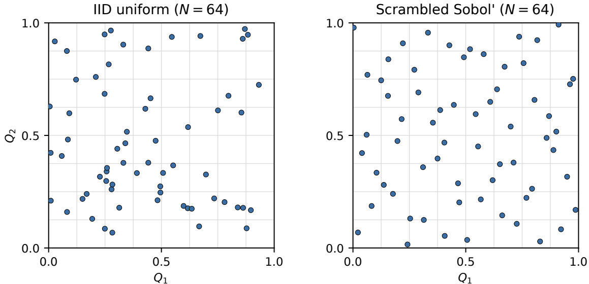
Figure 9.1: Comparison of N = 64 points in two dimensions. Left : independent identically distributed (IID) uniform samples show visible clusters and empty regions that waste model evaluations. Right : scrambled Sobol' sequence [37] achieves near-uniform coverage; every 8 \times 8 cell contains approximately one point. Both strategies produce marginally uniform samples, so both yield unbiased Sobol estimators; the LDS strategy produces much lower estimator variance for the same computational budget N .
