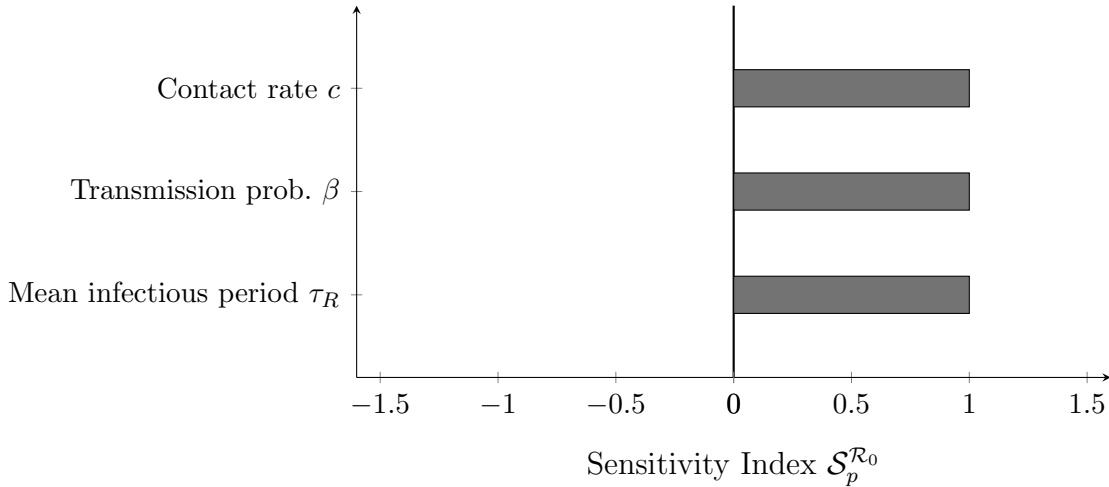
Figure 2.2: Tornado plot for the sensitivity of \mathcal{R}_0 to the three POIs of the SIR model, parameterized using interpretable durations and probabilities. All three indices equal +1, so the bars are equal in length and all extend to the right. In models with more parameters and a wider range of index values, the sorted layout reveals immediately which parameters dominate.
