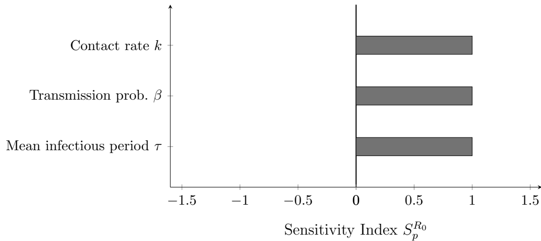
Figure 2.1: Tornado plot for the sensitivity of R_0 to the three POIs of the SIR model, parameterized using interpretable durations and probabilities. All three indices equal +1, so the bars are equal in length and all extend to the right. In models with more parameters and a wider range of index values, the sorted layout reveals immediately which parameters dominate.
