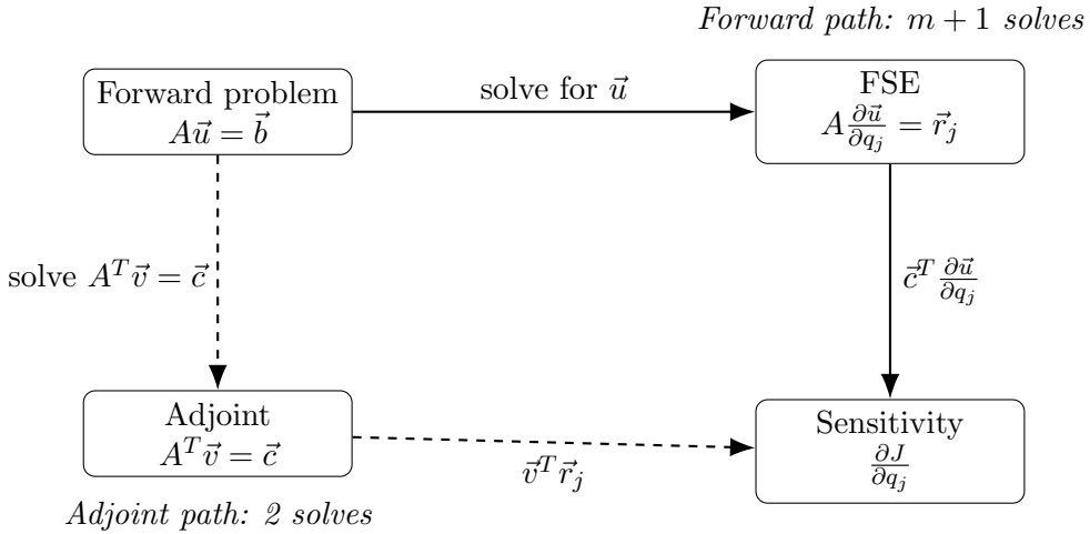
Figure 5.1. The commutative diagram for sensitivity analysis. The forward path (solid arrows) computes \partial J / \partial q_j by solving the FSE for each parameter, m + 1 solves total. The adjoint path (dashed arrows) solves the adjoint equation once, then evaluates the sensitivity formula for each parameter; 2 solves total. Both paths deliver the same result.
