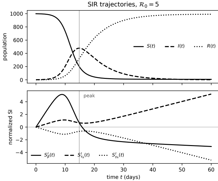
Figure 4.2. Forward sensitivity analysis of the SIR model via the FSE. Top: compartment trajectories at \mathcal{R}_0 = 5 . Bottom: time-dependent normalized sensitivity indices S_\beta^I(t) , S_{\tau_R}^I(t) , and S_{\gamma_R}^I(t) . Before the epidemic peak, transmission drives I(t) upward ( S_\beta^I, S_{\tau_R}^I > 0 ); after the peak, recovery dominates, and the plotted index S_{\tau_R}^I keeps growing, reaching +5.21 at t = 60 while S_\beta^I has turned negative. Stated in the recovery rate the same fact reads S_{\gamma_R}^I = -5.21 < 0 with magnitude increasing, since \gamma_R = 1/\tau_R flips the sign (§2.5); the figure plots the duration, not the rate. The sensitivity indices are not constant in time. The figure uses \mathcal{R}_0 = 5 rather than the chapter’s nominal \mathcal{R}_0 = c\beta\tau_R = 2.1 so that the post-peak regime is legible: at the nominal value the peak falls near day 44, as the Chapter 6 laboratory shows, leaving too little of a 60-day window after it to see the indices exchange rank. The qualitative behavior is the same at both values; only the timing changes.
