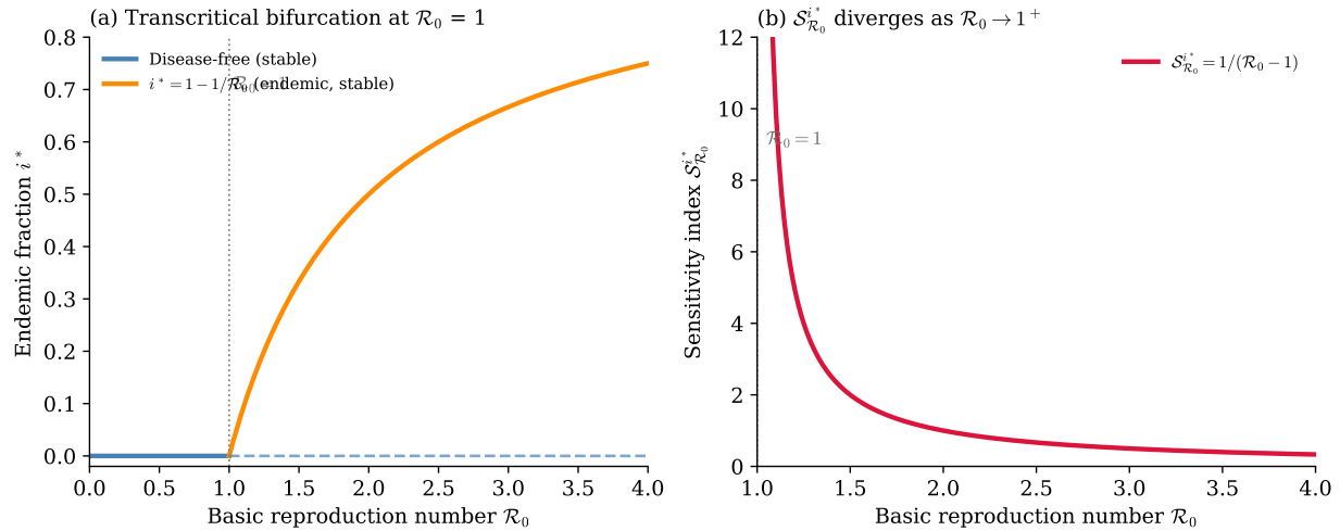
Figure 8.1: Bifurcation of the SIS endemic equilibrium at \mathcal{R}_0 = 1 . (a) The infectious fraction i^* = \max(0, 1 - 1/\mathcal{R}_0) : zero (disease-free state, stable) for \mathcal{R}_0 < 1 , rising continuously for \mathcal{R}_0 > 1 (endemic equilibrium, stable). The kink at \mathcal{R}_0 = 1 marks the transcritical bifurcation. (b) The sensitivity index \mathcal{S}_{\mathcal{R}_0}^{i^*} = 1/(\mathcal{R}_0 - 1) diverges as \mathcal{R}_0 \rightarrow 1^+ . Any parameter that shifts \mathcal{R}_0 near the epidemic threshold produces an arbitrarily large proportional change in the endemic level. Local SA correctly captures this infinite sensitivity but cannot predict the qualitative shift from disease-free to endemic behavior; that requires knowing that a bifurcation exists.
