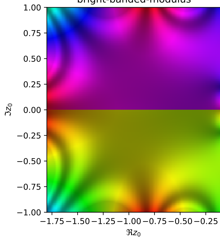
bright-banded-modulus
