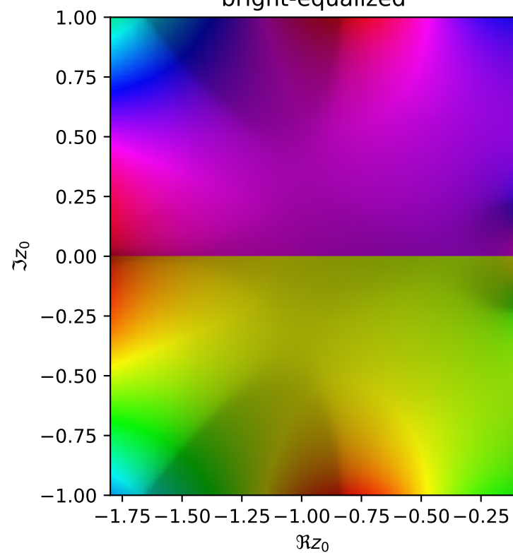
bright-equalized
