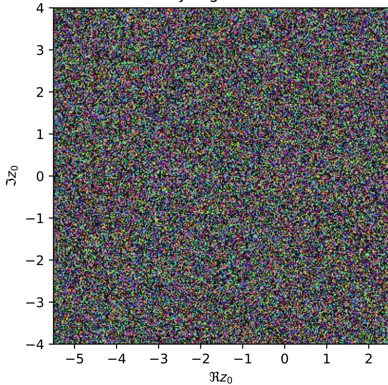
Naively regularized \Psi^{\circ 4}
