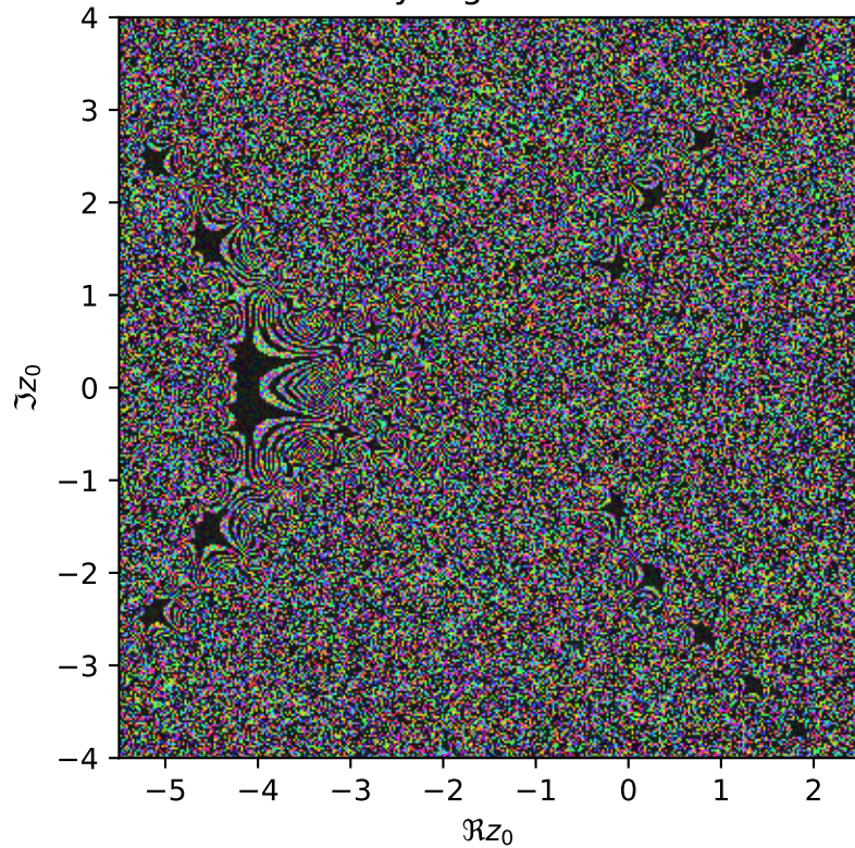
Naively regularized \Psi^{\circ 3}
