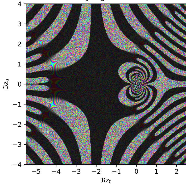
Naively regularized \Psi^{\circ 2}
