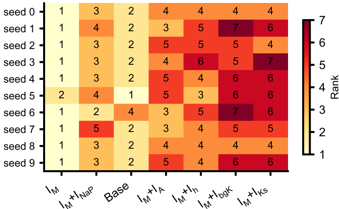
Family rank per seed (1 = best)
