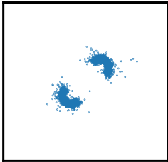
Repaint (r=0)
