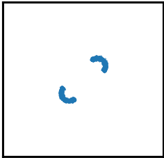
Conditional
