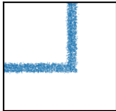
p(\theta|x_1 + x_2 = 0)
