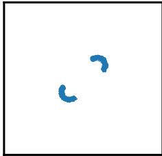
Repaint (r=5)
