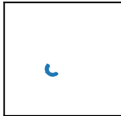
p(\theta|x, \theta < 0)
