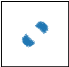
p(\theta|x \in [-0.1, 0.1])
