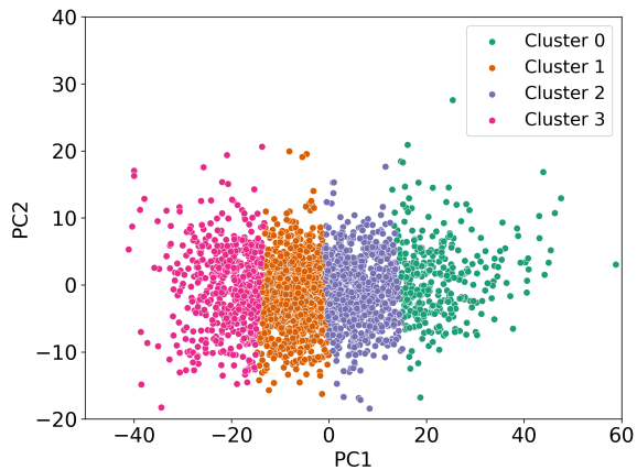
POPC-CHOL (Std + Halo Maps)
