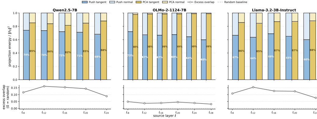
Figure 2: Projection energy \frac{\|P_{T_{h_\ell} \mathcal{M}} h_\ell\|^2}{\|h_\ell\|^2} of h_\ell in the approximated tangent space T_{h_\ell} \mathcal{M} for Qwen-2.5 7B, OLMo-2 7B, and LLaMA-3 3B. Below, we show the excess overlap between the pushforward tangent space and the PCA tangent space.
